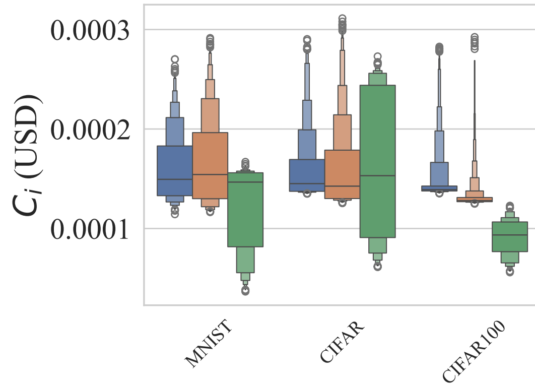
Inference Cost
