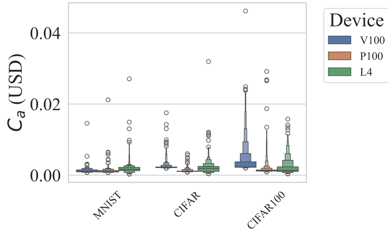
Attack Cost
