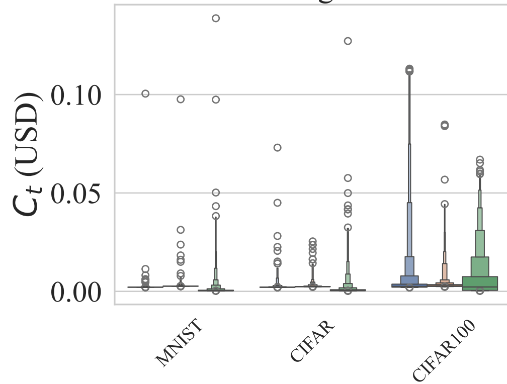
Training Cost
